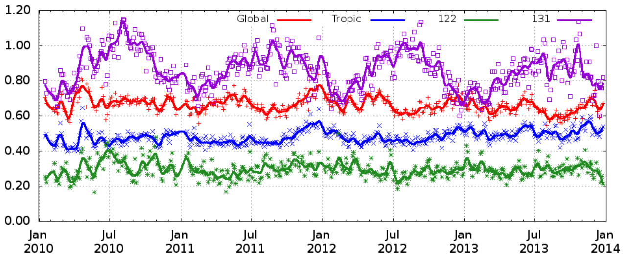
Fig 2: Standard deviation of SMOS minus ARGO SSS differences in 9-day binned maps for different ocean regions
